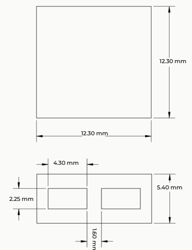
LEAD SEAL SQUARE
