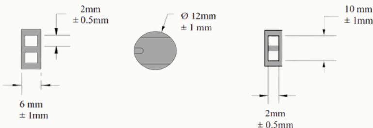
LEAD SEAL ROUND
